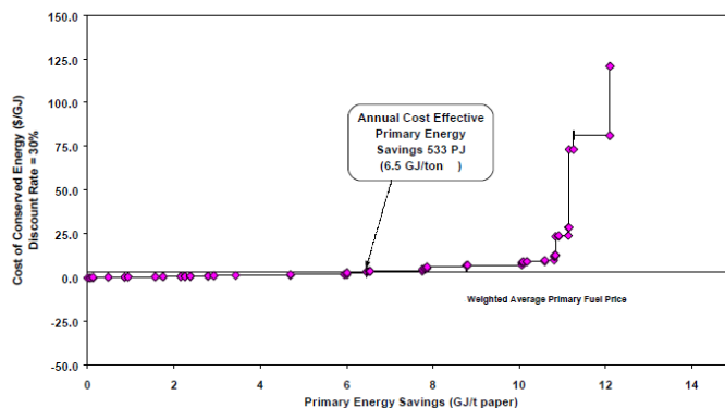
Figure 2 Energy Conservation Supply Curve for Thai Pulp and Paper Industry
