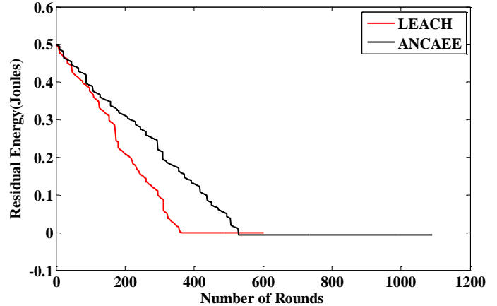
Figure 3 Average Residual Energy Vs number of rounds
