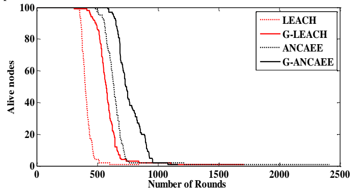
Figure 4 Alive nodes Vs Lifetime (in rounds)
