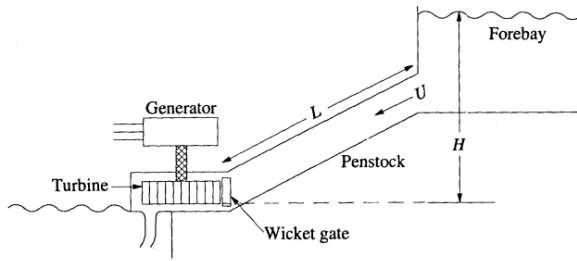
Fig.1 Schematic Diagram of Hydroelectric Plant
