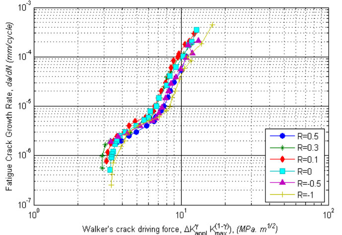
Fig. 4. FCG data in terms of Walker's crack driving force
