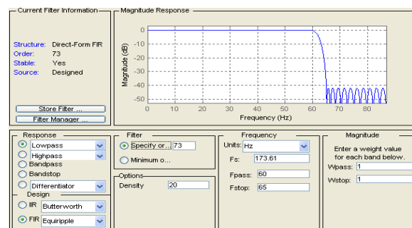
Fig.5. Magnitude response of FIR filter using Park-McClellan algorithm
