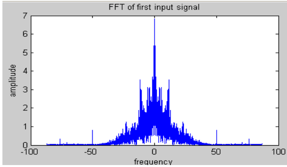
Fig.6. FFT of input with noise
