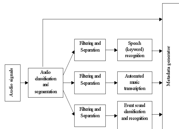
Figure 1. A typical high level metadata extraction system for audio tracks
