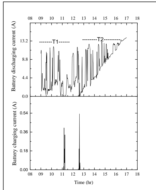
Figure 9. Battery charging and discharging current
