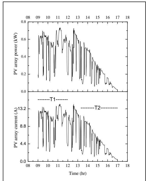
Figure 8. PV array power and current
