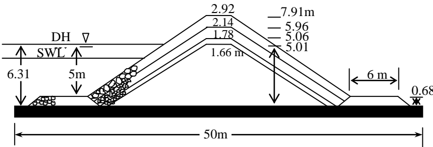
Fig. 9 Designed Cross Section of Groyne
