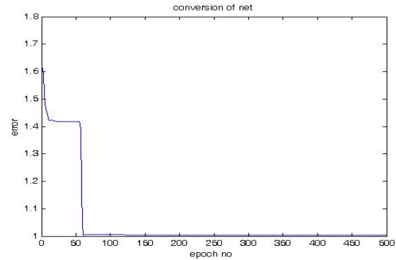
Fig 5. Learning Rate
