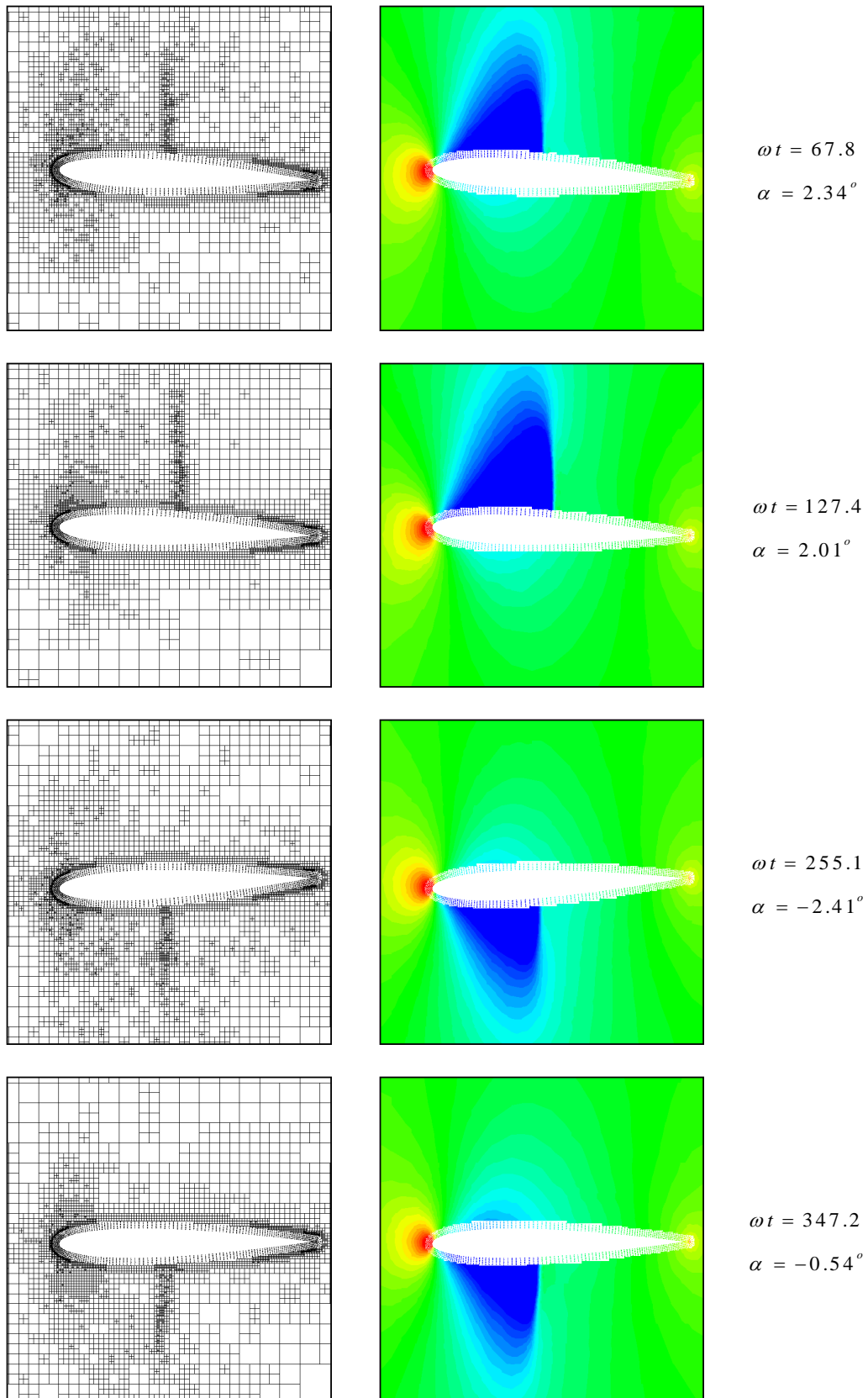
Figure 6. Instantaneous pressure contour and adapted grid with meshless zone for AGARD test case CT5.
