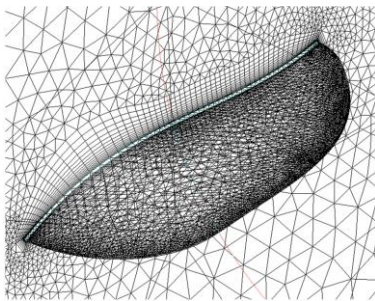
Figure 6. Elements for CFD analysis.
