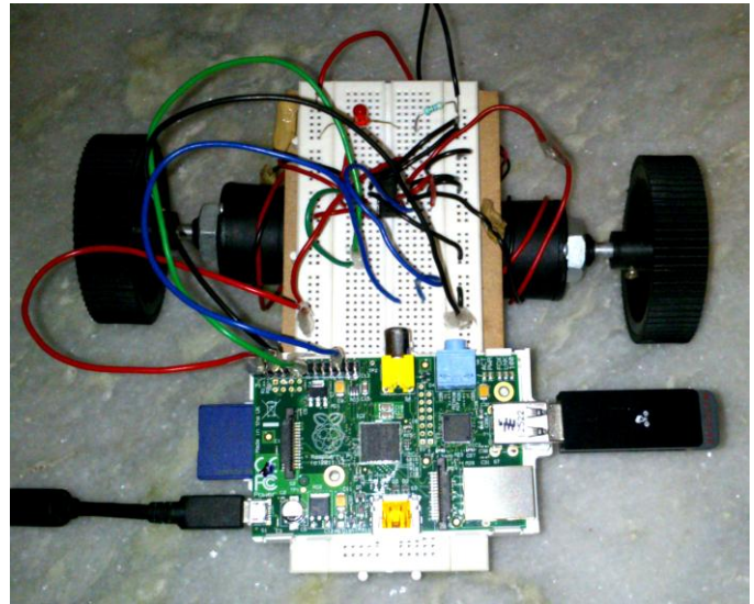
Figure 2. Electric Car with Onboard Computer
