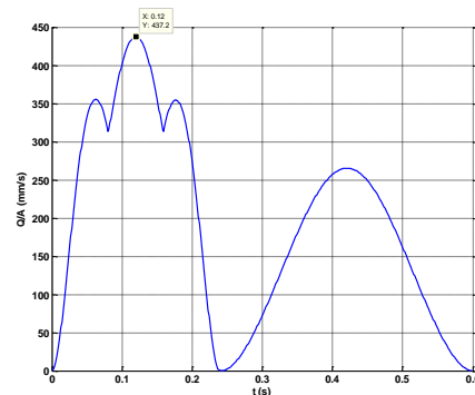
Figure 11. Flow rate Curve of One Leg
