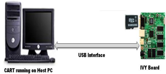
Fig 3: CART System
