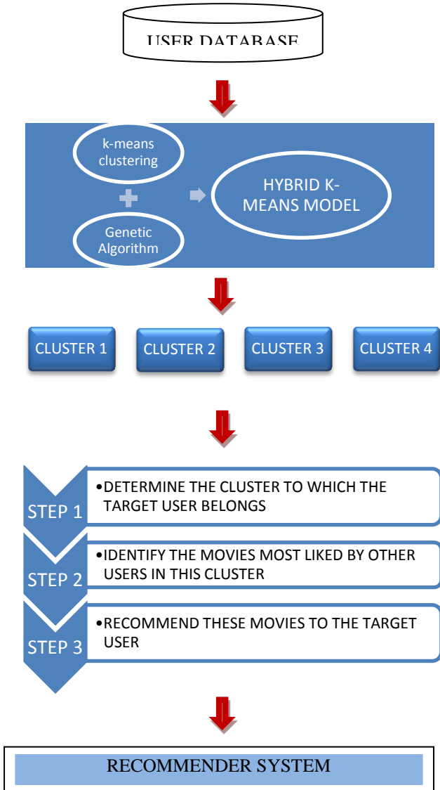
Fig 2: System Architecture of Recommender System
