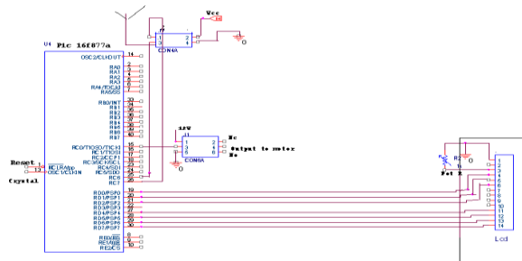
Fig.4. Circuit diagram of receiving section
