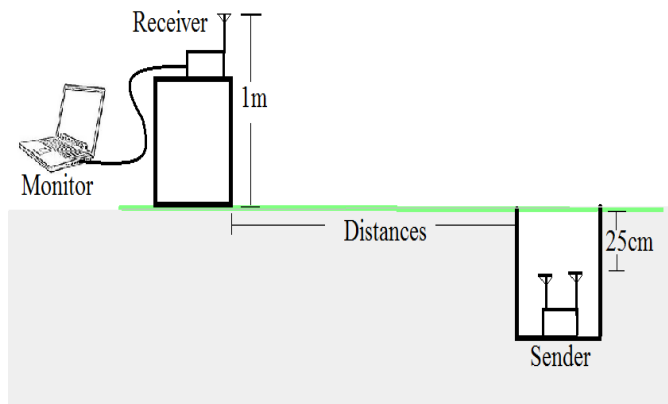
Figure 1. Experiments setup.
