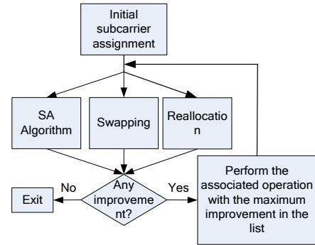
Fig. 3. Block diagram of the proposed allocation algorithms.
