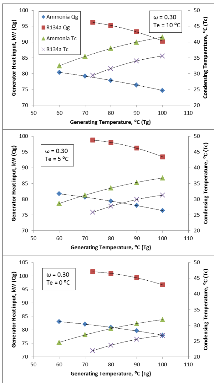
Figure 5. Effect of generating temperature to heat input and condensing temperature.
