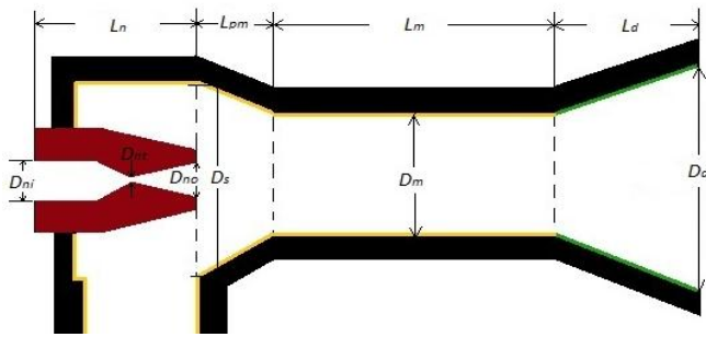
Figure 8. Ejector profile.
