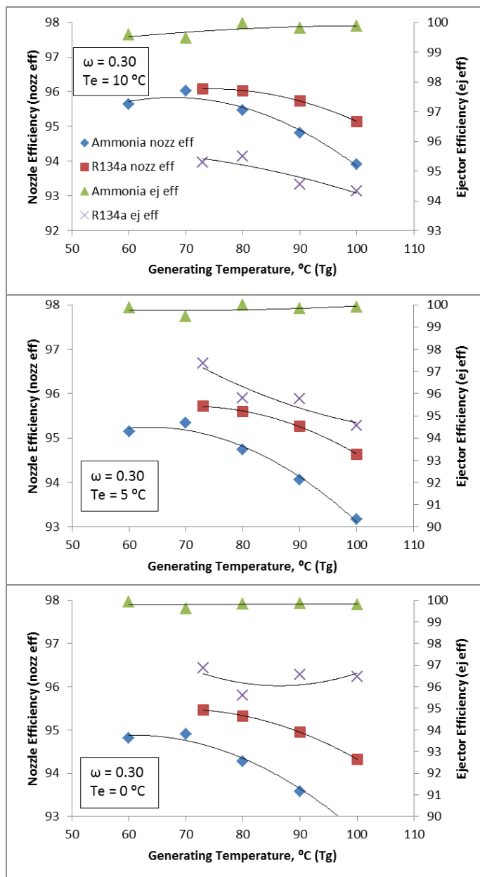
Figure 7. Effect of generating temperature to nozzle and ejector Efficiency.
