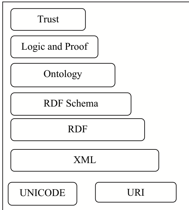
Fig.:1 Layered Architecture of Semantic web
