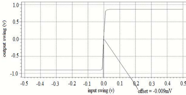
Figure 2. DC transfer curve
