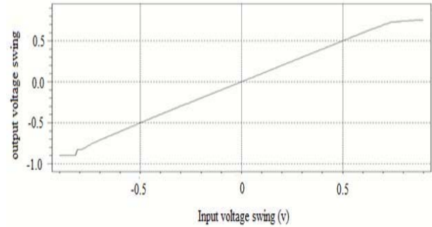
Figure 6. ICMR
