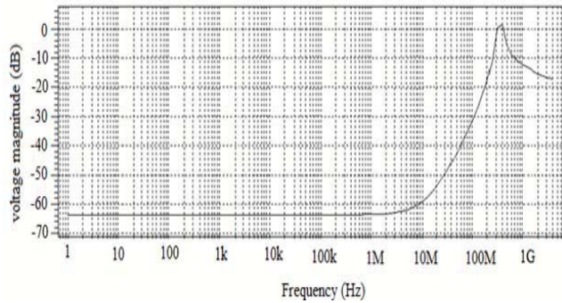
Figure 9. PSRR-
