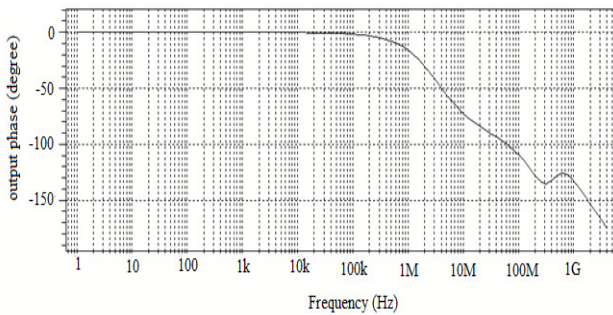
Figure 4. Phase vs frequency curve
