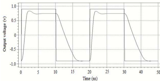
Figure 10. Slew rate of the op-amp
