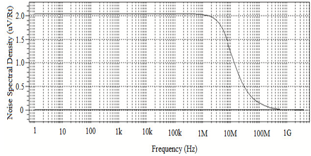
Figure 5. Output noise characteristics
