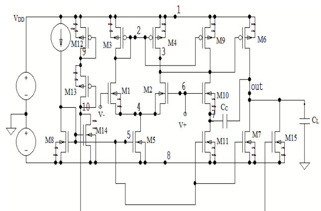
Figure 1. Circuit diagram of the proposed op-amp
