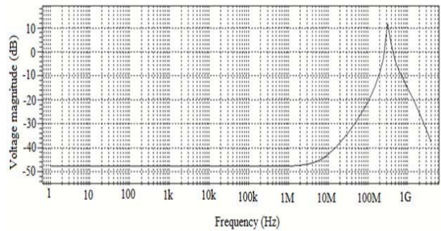
Figure 7. CMRR
