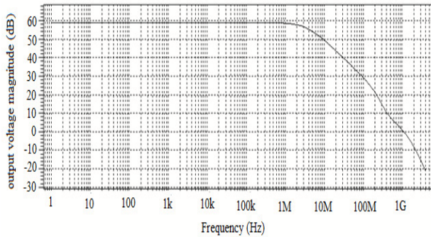
Figure 3. Gain vs frequency curve
