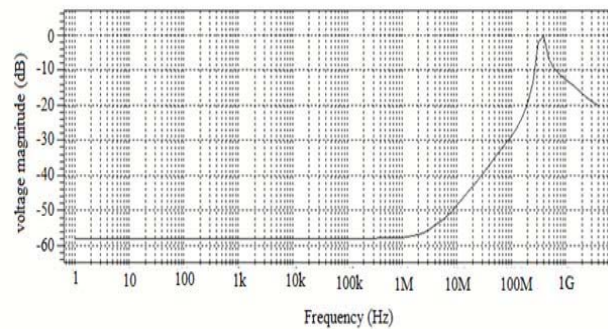
Figure 8. PSRR+
