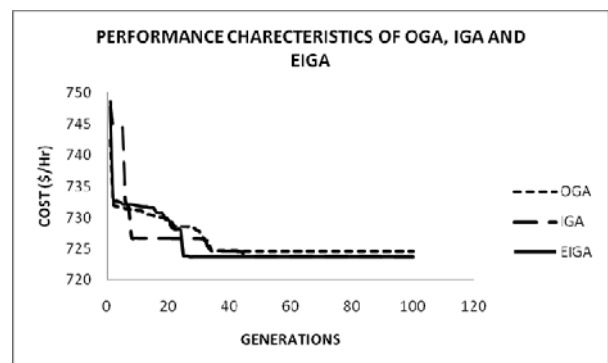
Figure 1. Performance of OGA, IGA and EIGA
