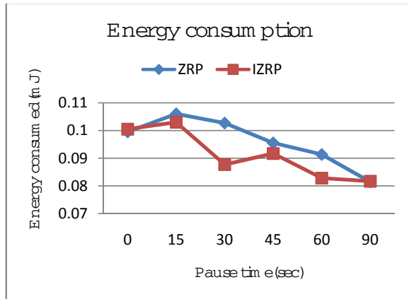
Figure 5. Energy consumption vs. Pause time
