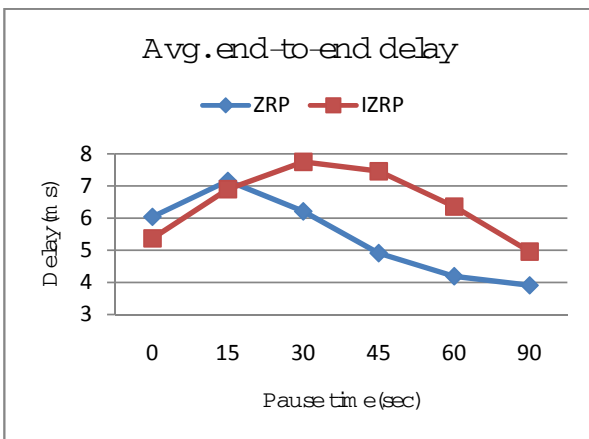
Figure 3. Avg. End-to-End Delay vs. Pause time
