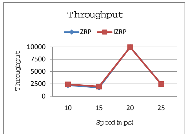
Figure 8. Throughput vs. Speed
