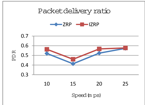
Figure 6. PDR vs. Speed
