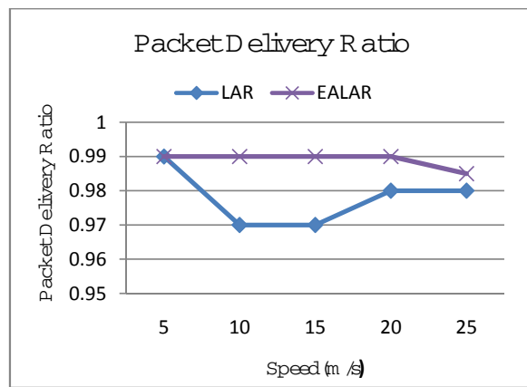
Figure 12. PDR vs. Speed
