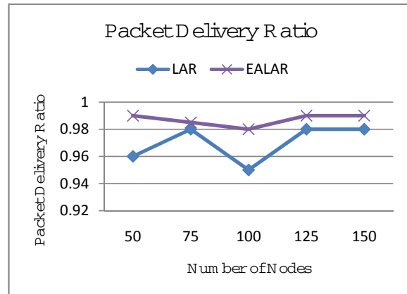
Figure 4. PDR vs. Number of Nodes
