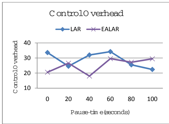
Figure 11. Control Overhead vs. Pause-time
