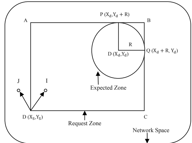
Figure 3. LAR1 scheme
