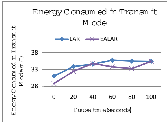
Figure 10. Energy Consumption vs. Pause-time
