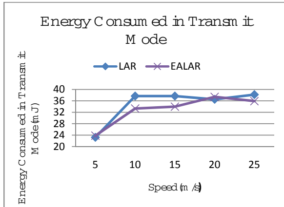
Figure 14. Energy Consumption vs. Speed
