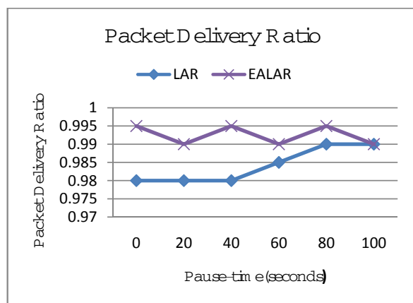
Figure 8. PDR vs. Pause-time
