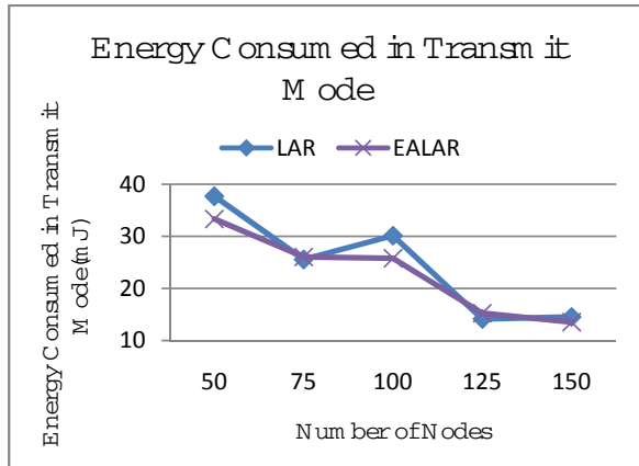
Figure 6. Energy Consumption vs. Number of Nodes
