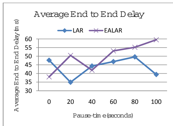
Figure 9. Average End to End Delay vs. Pause-time
