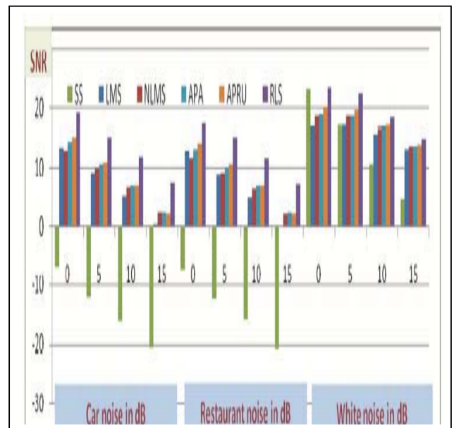
Figure 5. SNR comparison for SS, LMS, NLMS, APA, APRU and RLS algorithms
