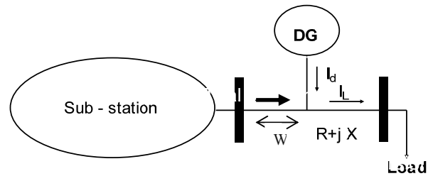
Fig.2 A distribution network with DG
