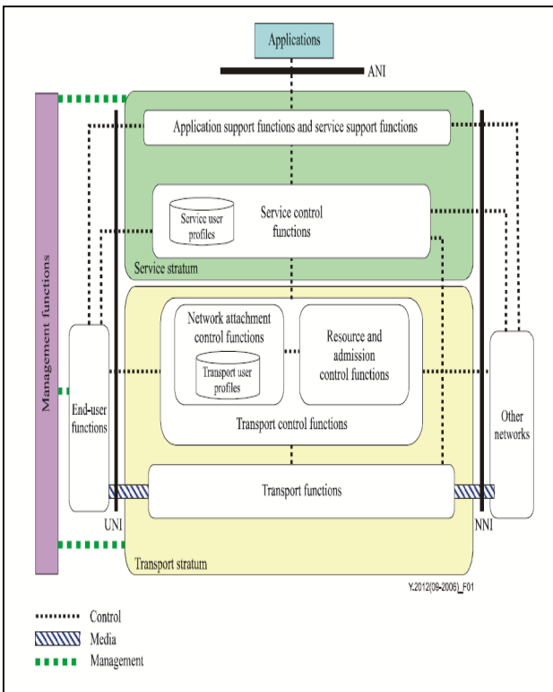
Figure 2 Architecture of NGN
