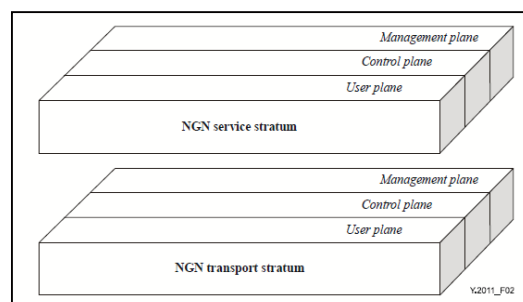
Figure 1 Layer and Planes in NGN Architecture
