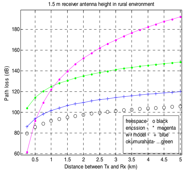
Fig 2 Pathloss for suburban area
