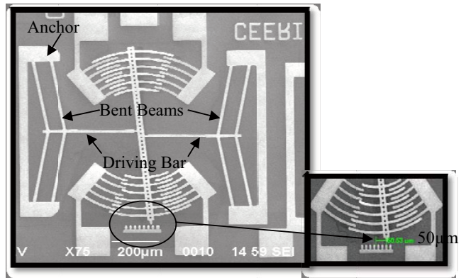
Figure 4. Symmetrical rotational type lancet structure with pointer and vernier for measure displacement due to material strain
