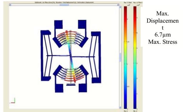
Figure 9 Simulated results of symmetric lancet structure used to determine the maximum stress and displacement
