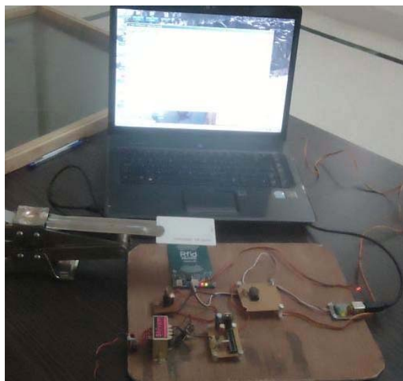
Fig 1.3 Setup for the observation
