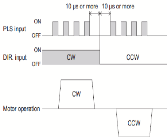
Figure 2. Controller waveform
