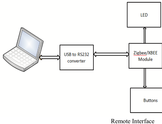
Figure 1. System Architecture
