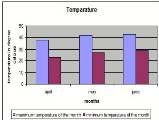
Figure 3 Maximum and minimum temperatures
