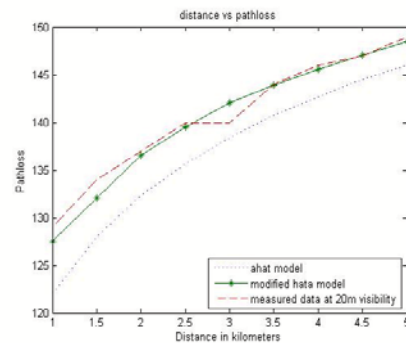
Figure 4 Path loss calculation at 20m visibility
