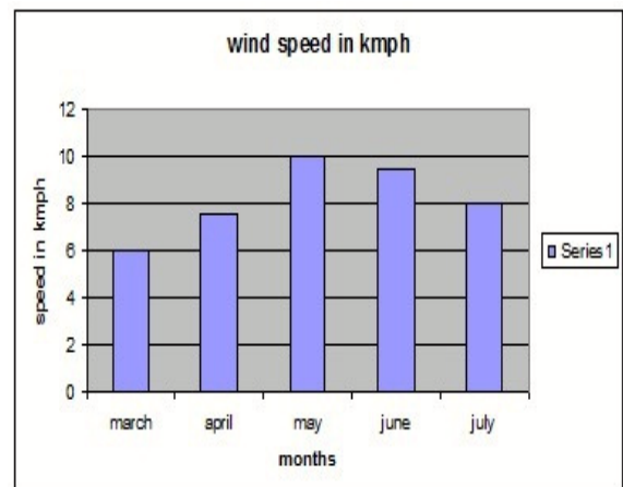
Figure 2 Average Wind speed
