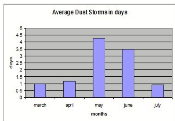
Figure 1 Average dust storm
