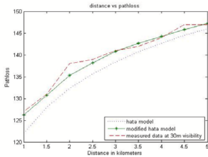
Figure 5 Path loss calculations at 30m visibility
