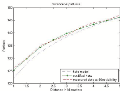
Figure 7 Path loss calculations at 50m visibility
