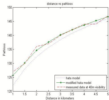
Figure 6 Path loss calculations at 40m visibility
