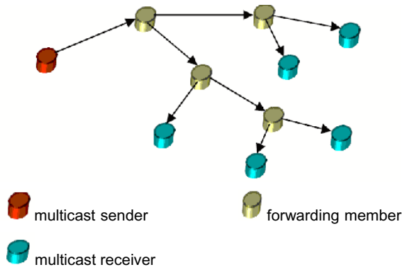
Figure 6: JOIN_DATA propagation
