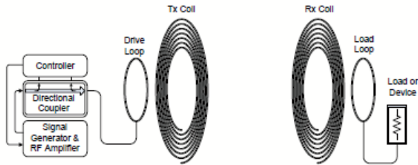
Fig. 5 Sketch of the magnetically coupled resonant wireless power system consisting of a RF amplifier, on the left, capable of measuring the forward and reflected power. A two element transmitter, made of a signal turn drive loop and high Q coil, wirelessly powers the receiver on the right.
