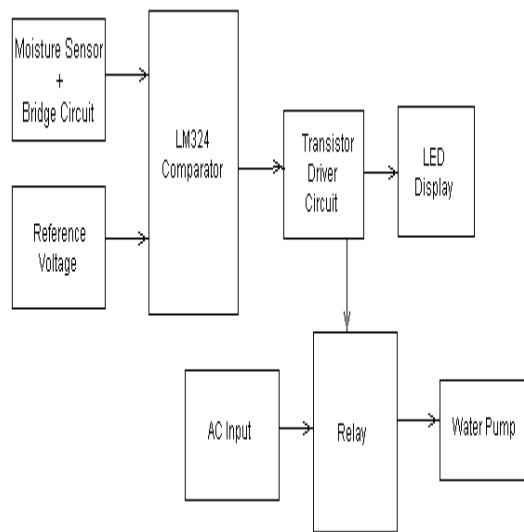
Figure2: Block diagram of the Set-Up
