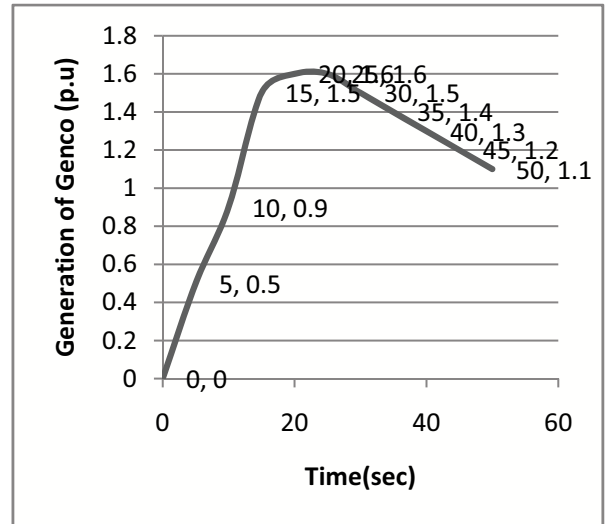
Fig 5 Characteristics of GENCOs of a hydro plant
