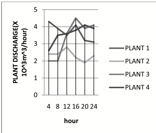
Fig 4. Hourly hydro plant Discharge
