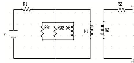
Figure 7. Equivalent circuit diagram of fig.-3
