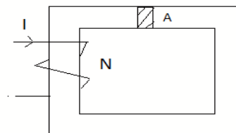
Figure 1. Magnetic Circuit
