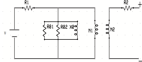
Figure 6. Equivalent circuit diagram of fig.-2
