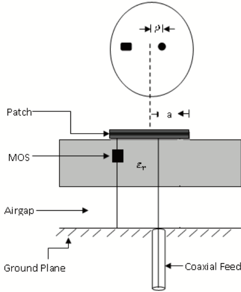
Fig. 1 Structure of a MOS loaded circular microstrip antenna with airgap
