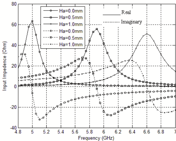
Fig. 4 Variation of Input Impedance with frequency of circular microstrip antenna with different airgap
