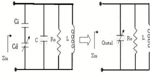
Fig.3 Equivalent circuit of MOS loaded circular microstrip antenna
