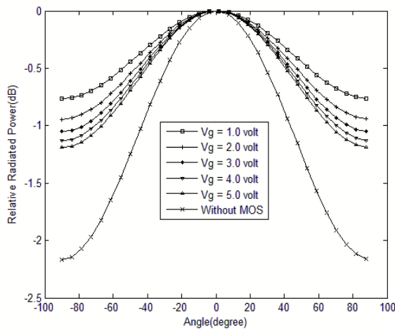
Figure 11: H-plane radiation pattern of MOS loaded circular microstrip antenna with airgap ( H_a = 1.0 mm)
