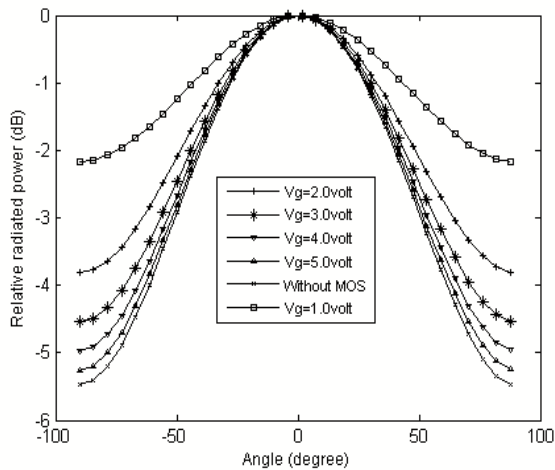
Fig. 10 E-plane radiati on pattern of MOS loaded circular microstrip antenna with airgap ( H_a = 1.0 mm)
