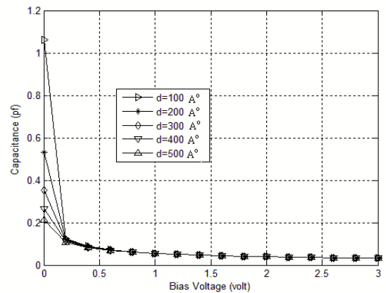
Fig.5 Variation of capacitance of a MOS with bias voltage
