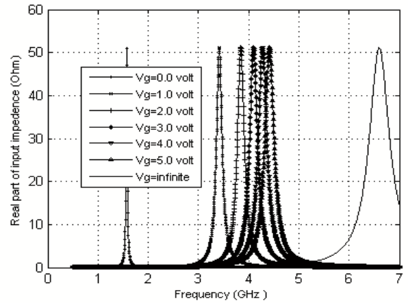
Fig.8 V variation of input impedance with frequency with different bias voltage ( V_g ) of MOS loaded circular microstrip antenna with airgap ( H_a = 1.0 mm)
