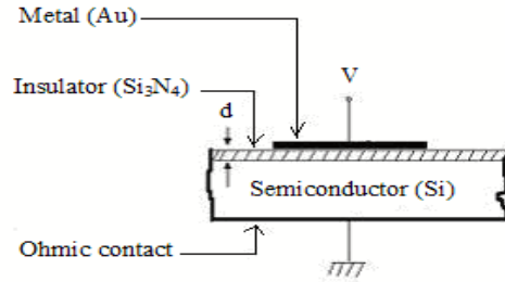
Fig. 2 Schematic of MOS capacitor
