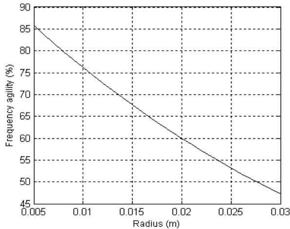
Fig.7 V variation of frequency agility with radius of patch of MOS loaded circular microstrip antenna with airgap ( H_a = 1.0 mm)
