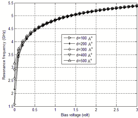
Fig.6 Variation of resonant frequency with bias voltage of MOS loaded CMSA with airgap
