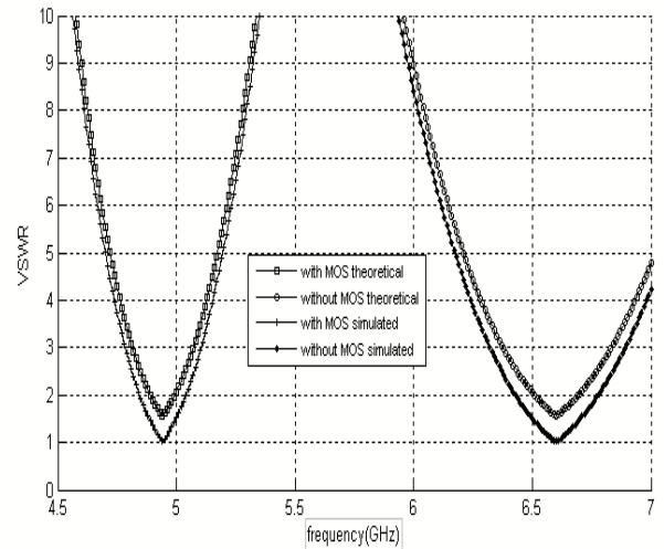
Fig. 9 Variation of VSWR with and without MOS circular microstrip antenna with airgap ( H_a = 1.0 mm)
