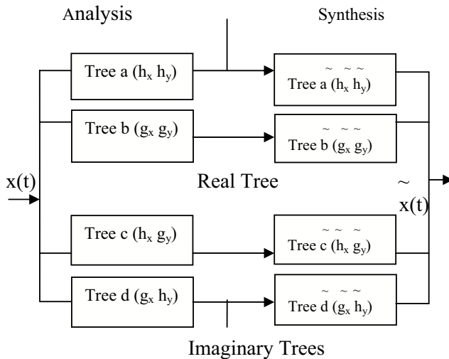
Figure (5) Filter bank structure for 2-D DT-DWT
