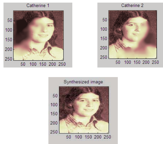
Figure (7) Image Fusion and De-noised Image Using DWT
