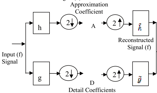
Figure(2) One Dimensional Wavelet Analysis and Synthesis Filters
