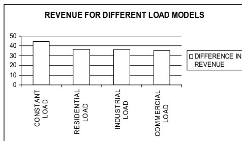
Figure 1: Revenue for different load models
