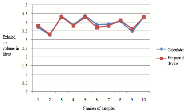
Figure 9: A comparative graphical display of FEV1 values between the normal reference calculator and proposed spirometer
