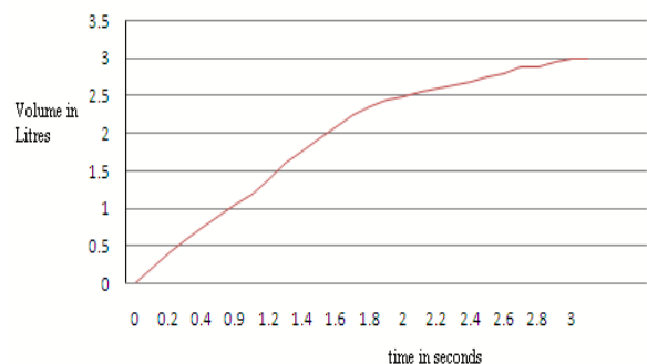
Figure5: Obstructive volume-time curve
