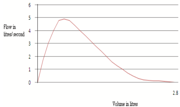
Figure 8: Restrictive exhaled flow-volume curve
