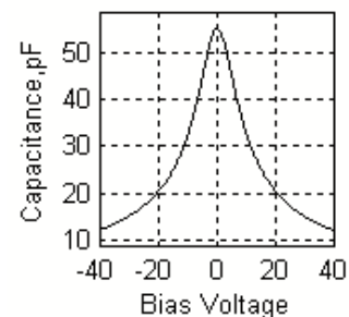
Figure 6: Variation of capacitance with bias voltage
