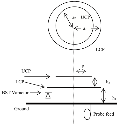
Figure 1. Structure of proposed antenna
