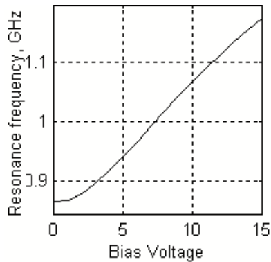
Figure 8. Variation of resonant frequency with bias voltage
