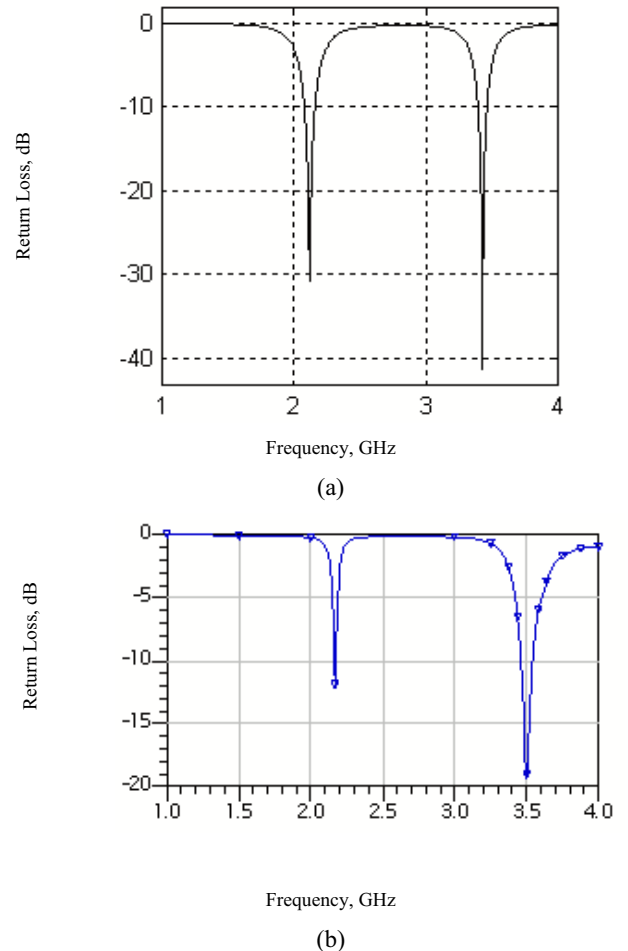
Figure 5. Return loss of Stacked CMSA (a) Calculated (b) Simulated
