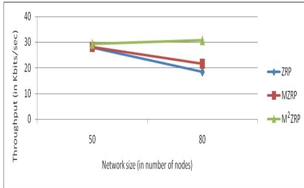
Figure 3: Throughput comparison using Random Way Point (RWP) node mobility model.
