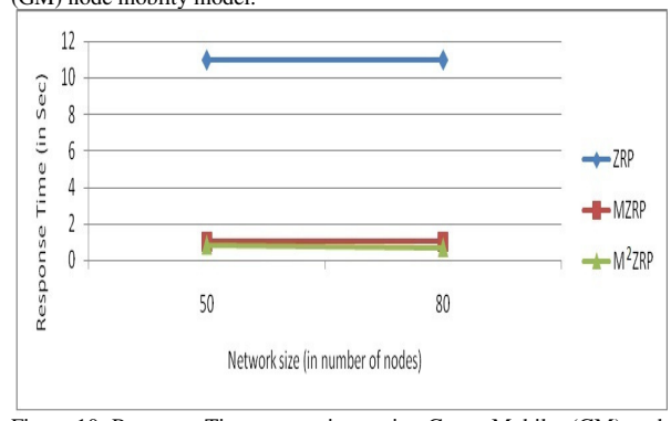
Figure 10: Response Time comparison using Group Mobility (GM) node mobility model.
