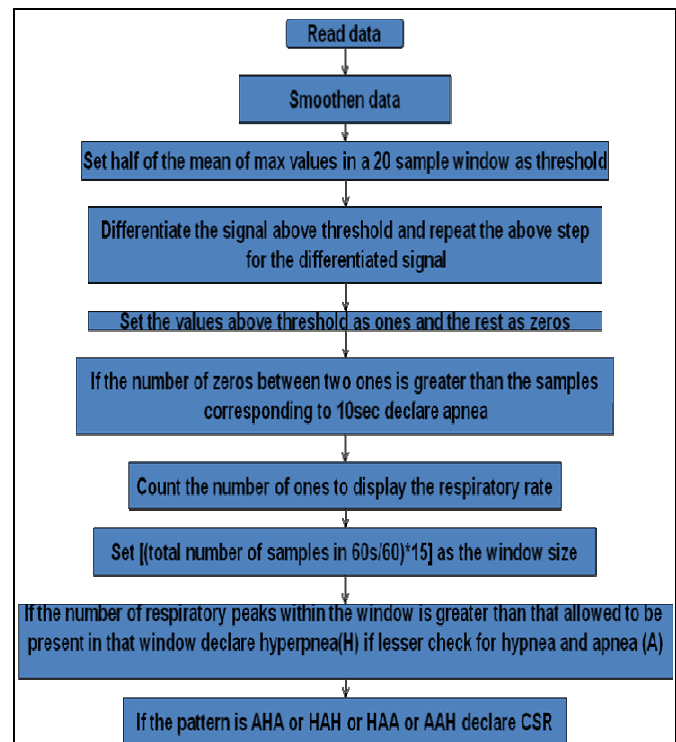
Fig.2. Detection of CSR and respiratory rate measurement
