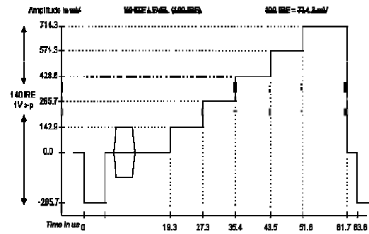
Figure 6 : Grey scale Standard wave form
