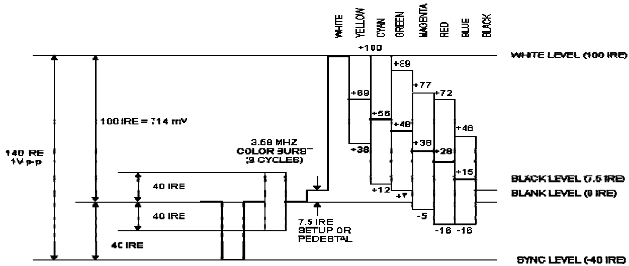
Fig. 4 Colour Signal Wave form
