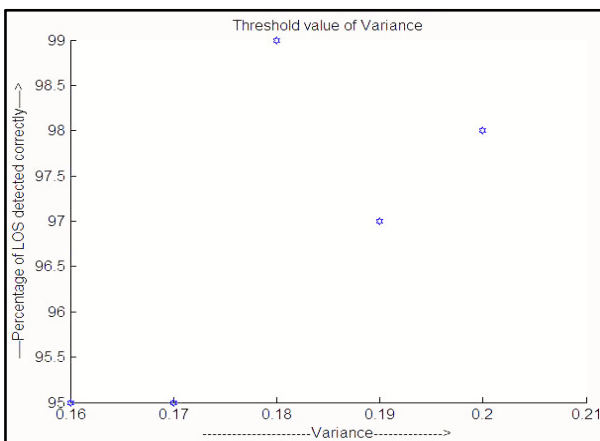
Figure 1: Determining Threshold of variance of RSS value for LOS condition
