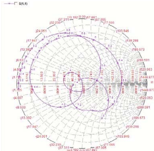
Fig.8. Smith Chart of proposed geometry of octagonal Microstrip Patch Antenna.
