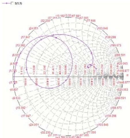
Fig.5. Smith Chart of octagonal Microstrip Patch Antenna
