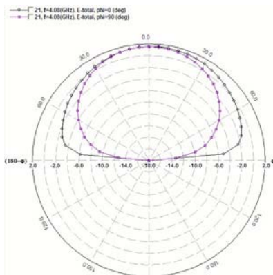
Fig.6. 2D Radiation Pattern for proposed geometry of octagonal Microstrip Patch Antenna.
