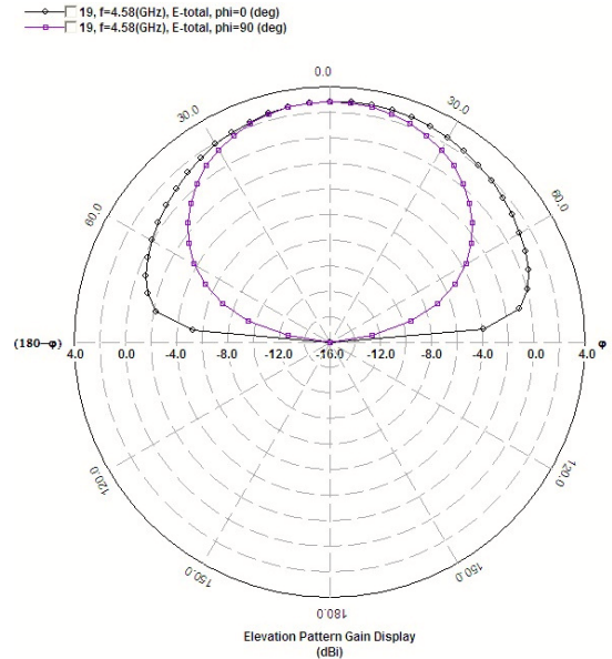
Fig.3. 2D Radiation Pattern for octagonal MPA
