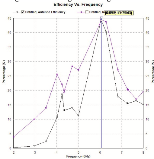
Fig.9. Efficiency graph of proposed geometry of octagonal Microstrip Patch Antenna.
