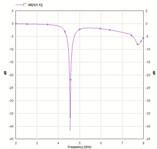
Fig.4. Simulated Return Loss for octagonal Microstrip Patch Antenna.
