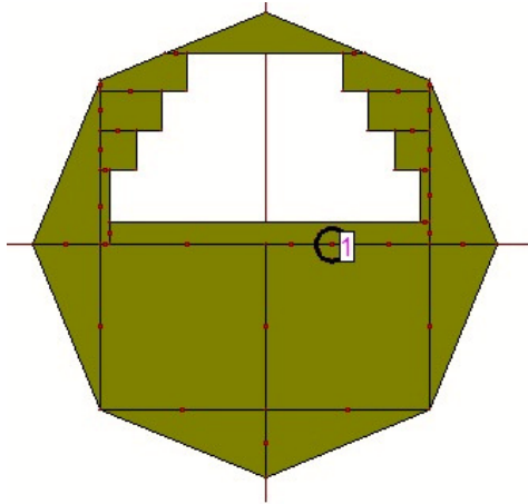
Fig.2. Proposed geometry of octagonal MPA
