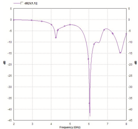
Fig.7. Simulated Return Loss for proposed geometry of octagonal Microstrip Patch Antenna.
