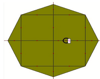
Fig.1. Octagonal Microstrip Patch Antenna.
