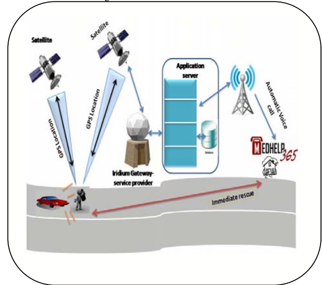
Figure 1: Architecture of EmerSat.
