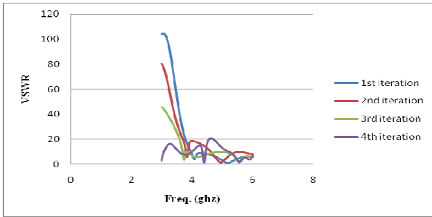
Figure 7. VSWR for I to IV iterations
