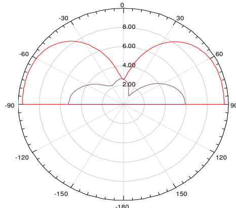
Figure 11. Radiation Pattern for IVth iteration
