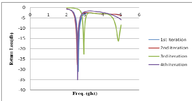
Figure 9. Return loss for I to IV iterations
