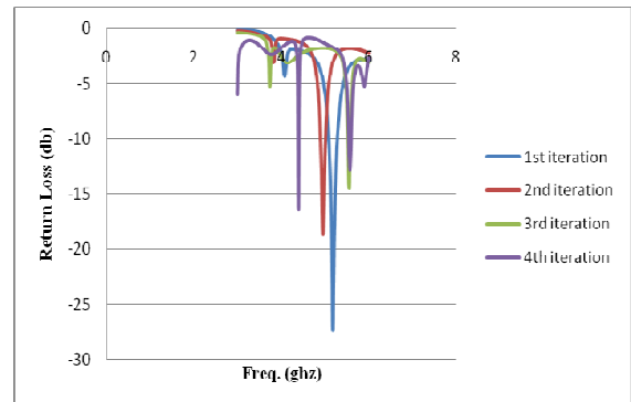
Figure 6. Return loss for I to IV iterations
