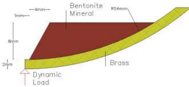
Figure 2. Illustration of Slope Modeling.
