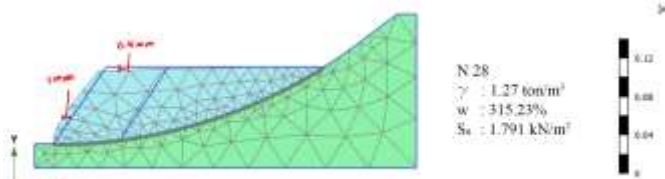
Figure 12. Numerical Output (28 Blows).
