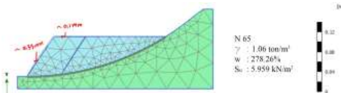
Figure 13. Numerical Output (65 Blows).
