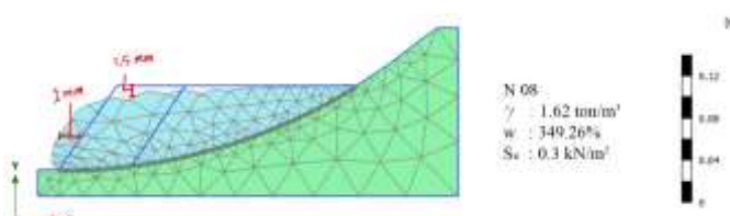
Figure 11. Numerical Output (8 Blows).
